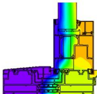
distribution of isotherms in the MB-77HS HI window
